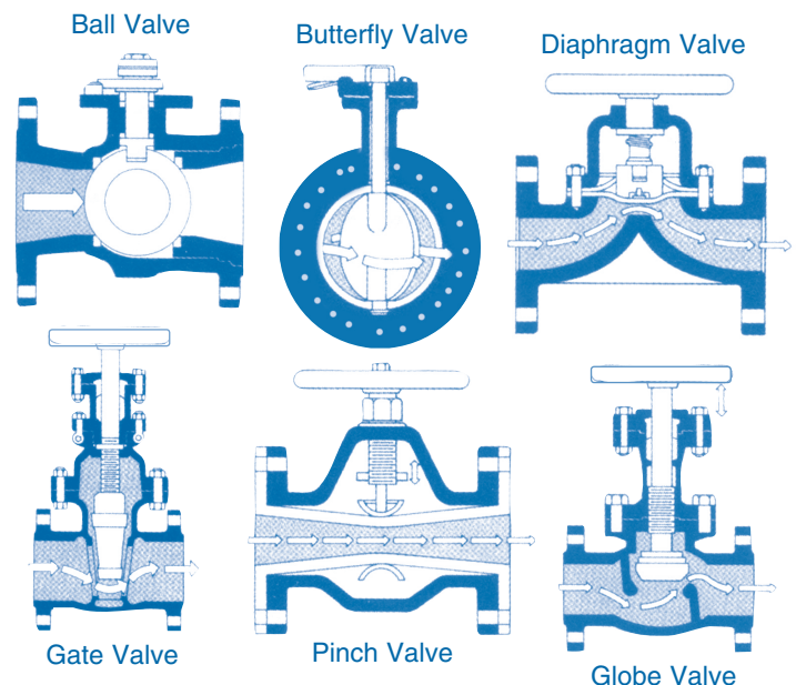
Figure 1 - Manual Valves
