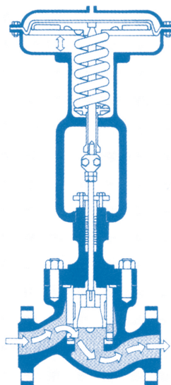
Control Valve
