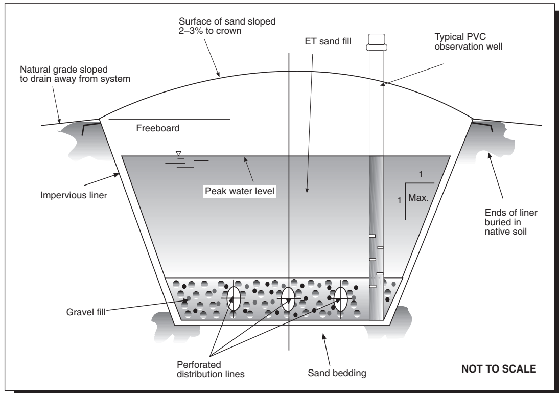
Figure 1: Cross Section of a Typical Evapotranspiration Bed
