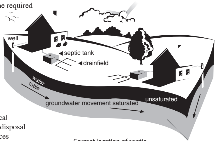
Correct location of septic systems and drinking water wells
