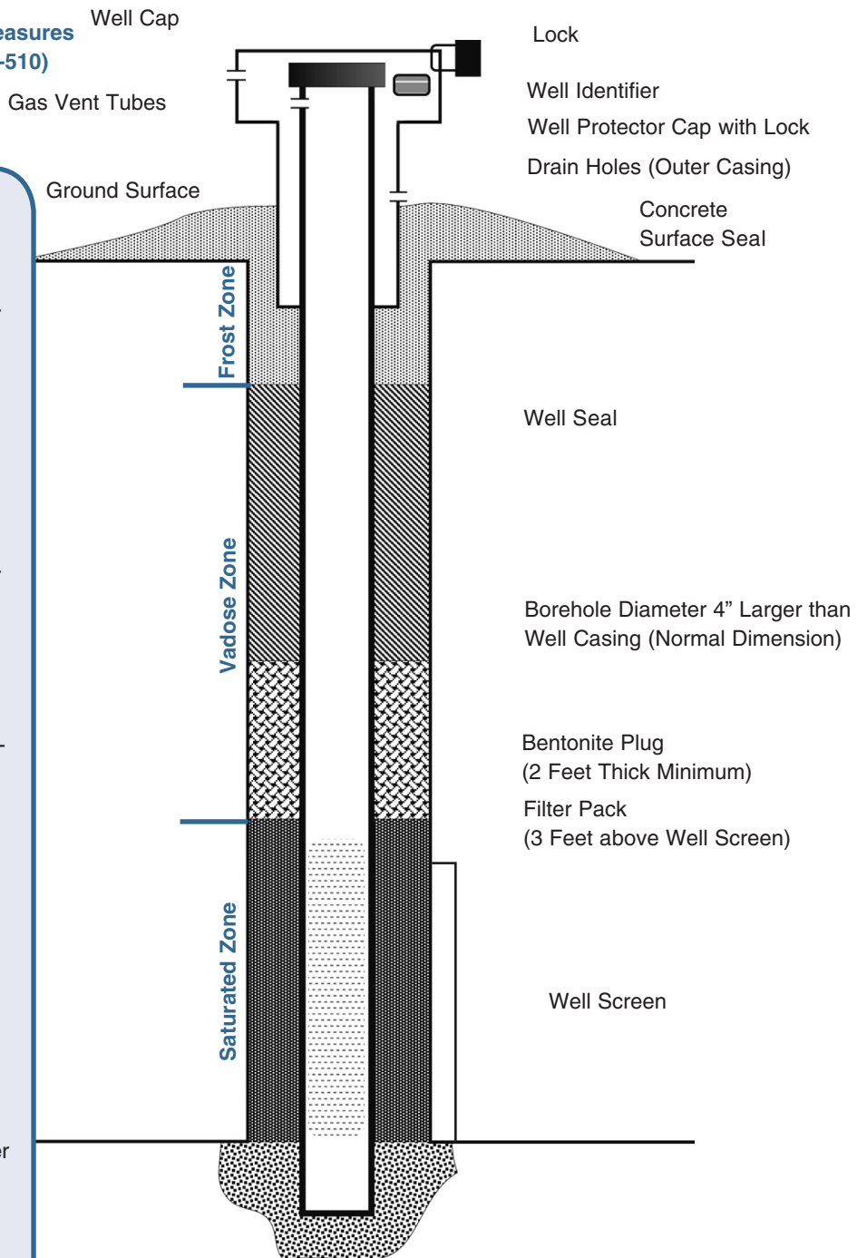
Figure 1: General Resource Protection Well–Cross Section
