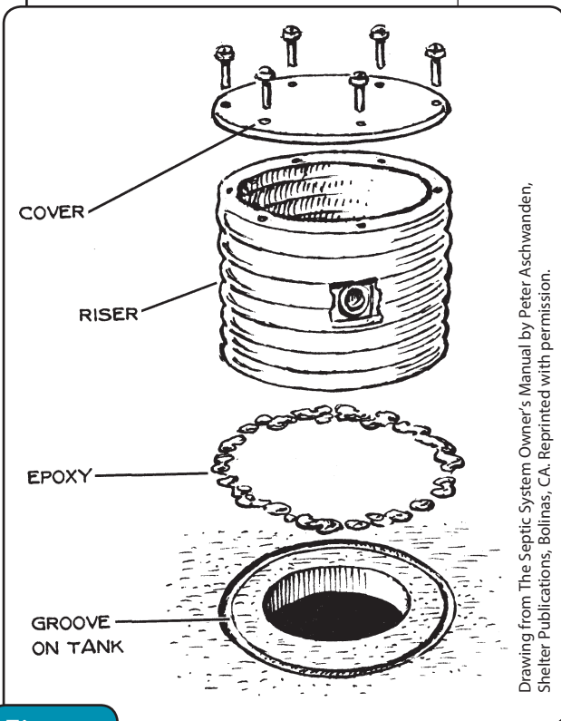
Figure Detail for retrofitting a riser on an existing tank.
