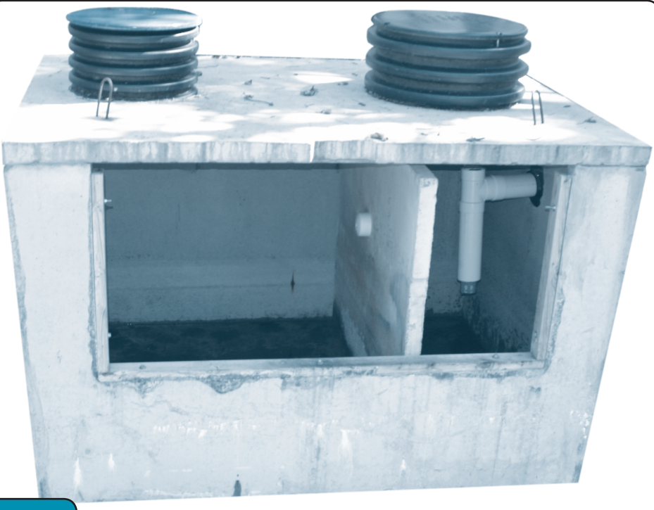
Figure Cutaway view of a dual compartment concrete tank.
