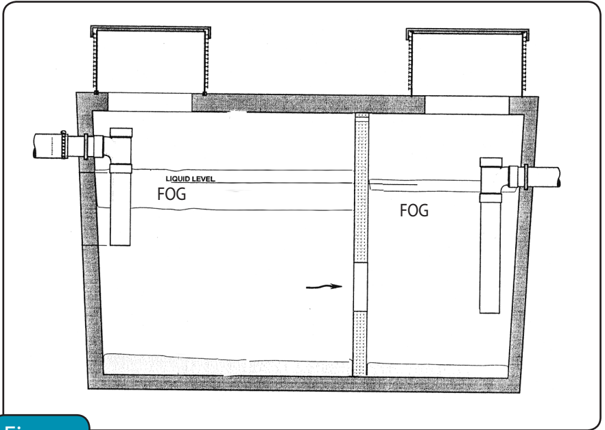
Figure Diagram of a typical grease trap.
