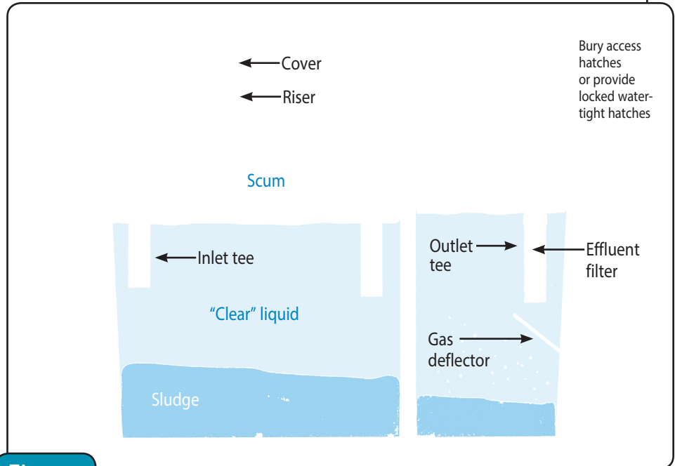
Figure Diagram of a typical dual compartment tank.
